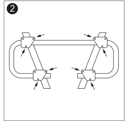
The most common mounting of the bottom frame.
