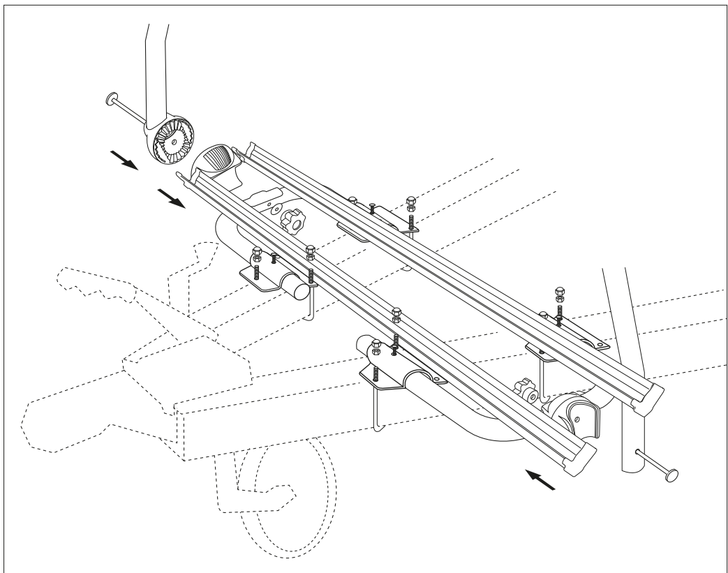
The top frame of the bicycle carrier can be tilted forward; as a result, the drawbar of the caravan remains accessible when the bicycle carrier is mounted.
