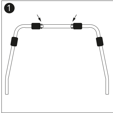
Before the top frame is placed on the support frame, it must first be mounted.
