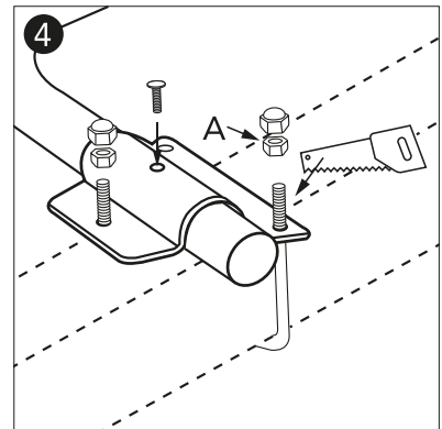
The height of the frame of the drawbar determines the cutting of the thread. Tighten the nut (A) first before cutting!
